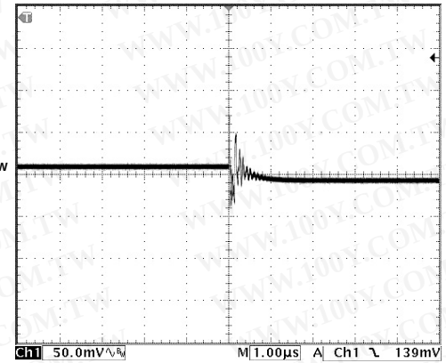
Figure 25. Midscale Glitch, Code 0x80 to Code 0x7F
