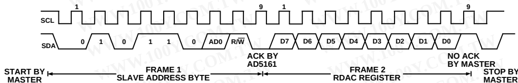
Figure 41. Reading Data from a Previously Selected RDAC Register in Write Mode
