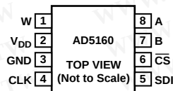
Figure 3. Pin Configuration
