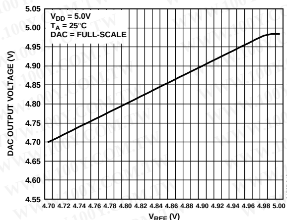
Figure 27. Output Voltage vs. Reference Voltage
