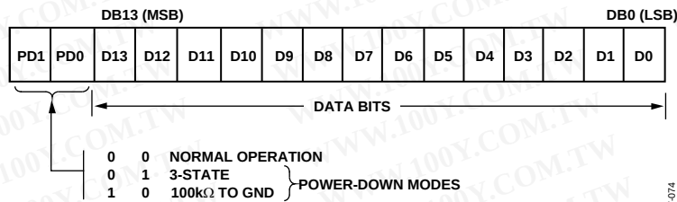
Figure 42. AD5040 Input Register Content
