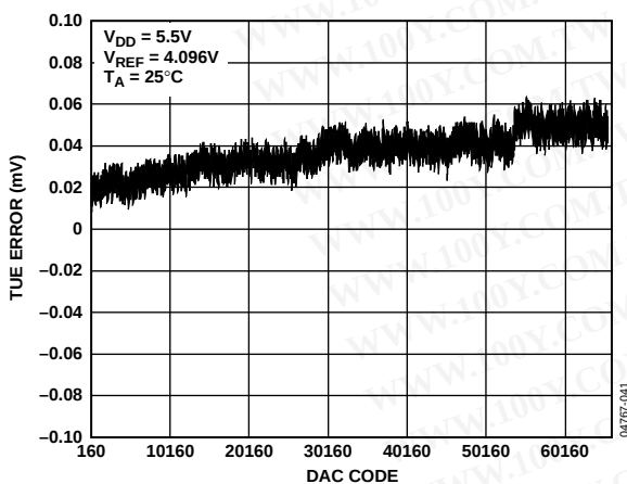
Figure 6. Typical AD5060 TUE Plot
