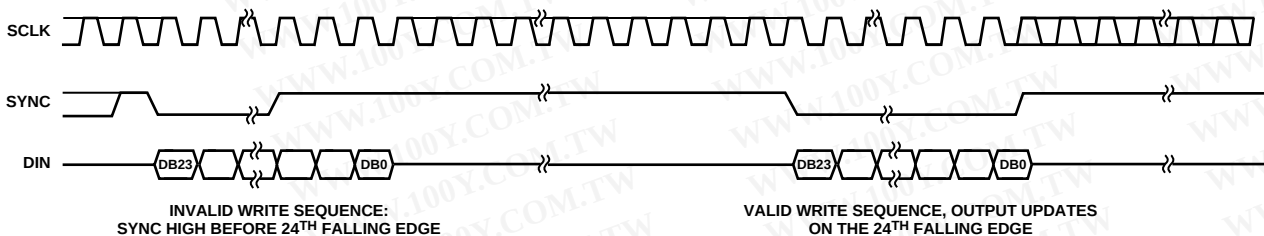
Figure 43. AD5060 SYNC Interrupt Facility
