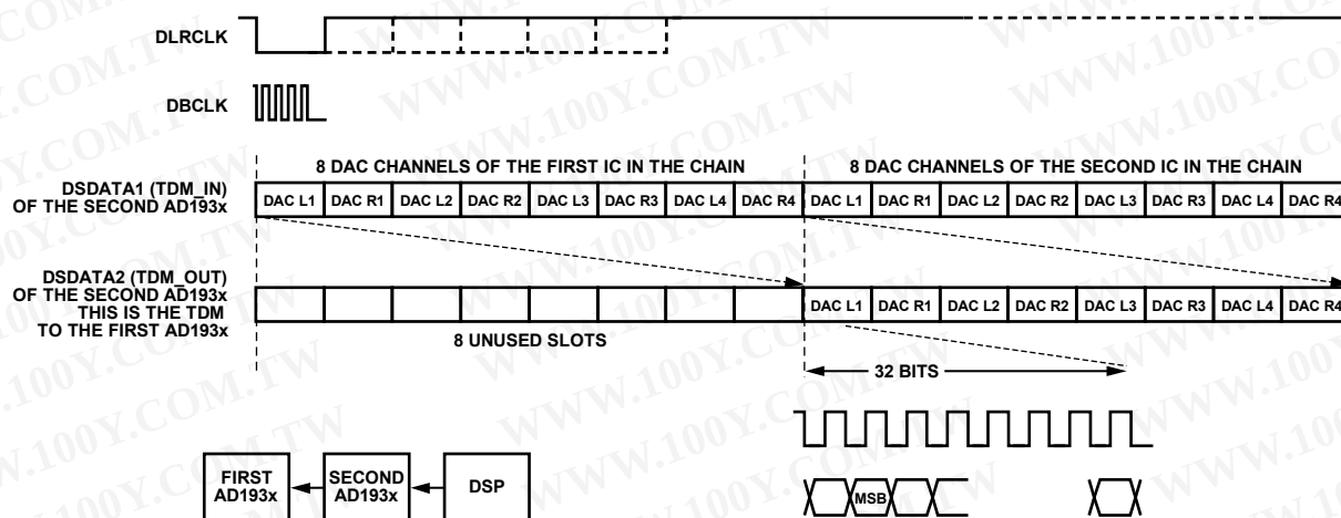
Figure 18. Single-Line DAC TDM Daisy-Chain Mode (Applicable to 48 kHz Sample Rate, 16-Channel, Two-AD1938 Daisy Chain)
