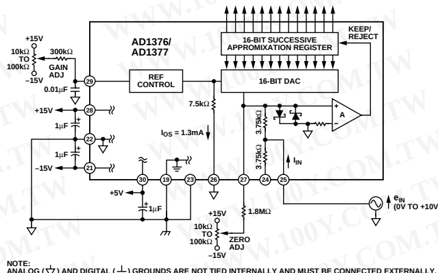
Figure 11. Analog and Power Connections for Unipolar 0 V to 10 V Input Range
