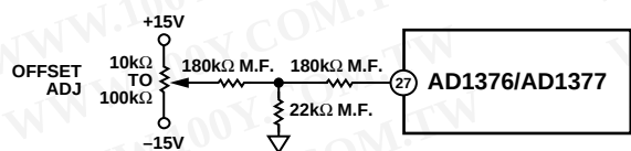
Figure 7. Low Temperature Coefficient Zero Adjustment Circuit
