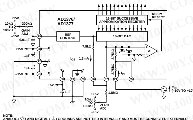
Figure 12. Analog and Power Connections for Bipolar -10 V to +10 V Input Range
