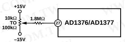
Figure 6. Zero Offset Adjustment Circuit ( \pm 0.3\% FSR)
