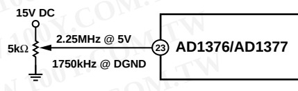
Figure 13. Clock Rate Control Circuit
