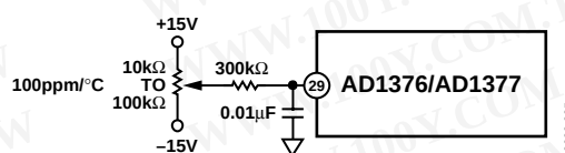
Figure 5. Gain Adjustment Circuit ( \pm 0.2\% FSR)
