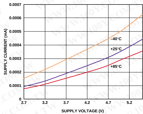
Figure 14. AD7994 Shutdown Current vs. Supply Voltage, -40^{\circ}\text{C} , +25^{\circ}\text{C} , and +85^{\circ}\text{C}
