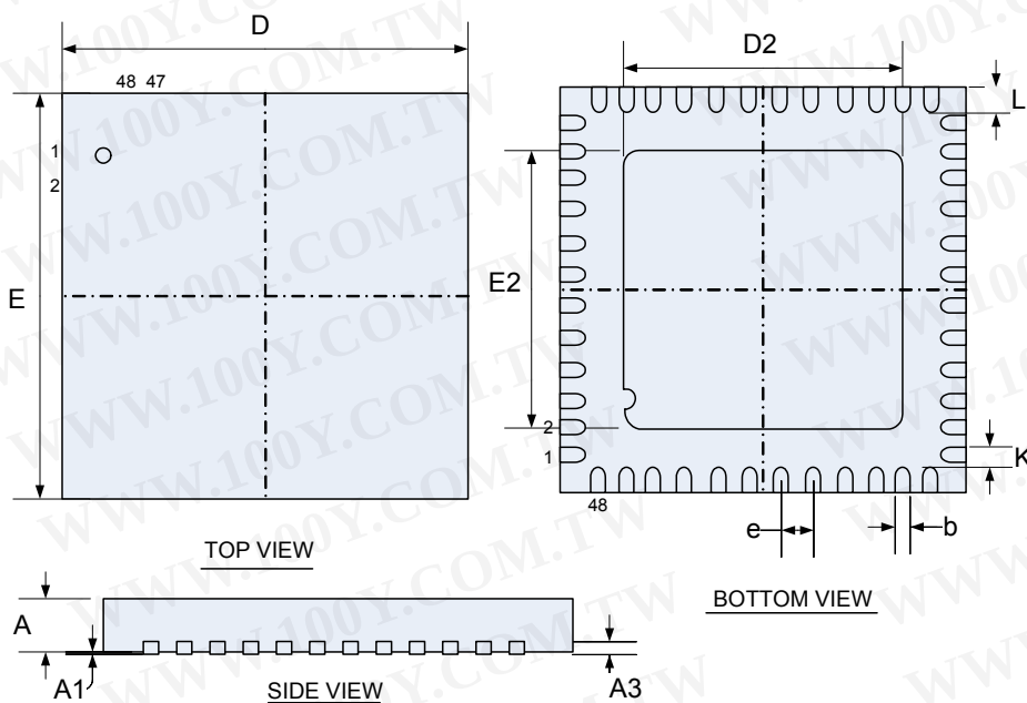
Figure 78. QFN48 pin 7×7mm
