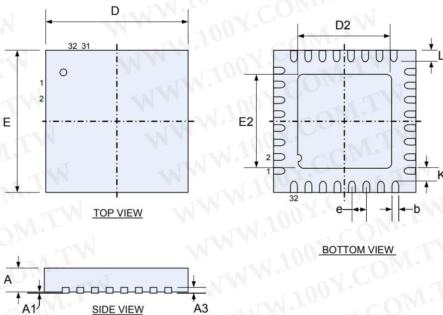
Figure 77. QFN32 pin 5×5mm
