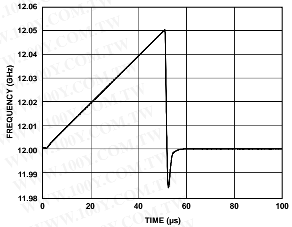
Figure 9. Sawtooth Burst, f_{PD} = 100 MHz, I_{CP} = 2.5 mA, Loop Bandwidth = 250 kHz, CLK_1 = 3 , CLK_2 = 26 , DEV = 1024 , DEV\_OFFSET = 8 , Number of Steps = 64
