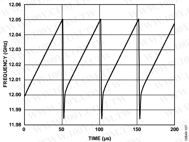
Figure 7. Sawtooth Ramp, f_{PD} = 100 MHz, I_{CP} = 2.5 mA, Loop Bandwidth = 250 kHz, CLK_1 = 3 , CLK_2 = 26 , DEV = 1024 , DEV\_OFFSET = 8 , Number of Steps = 64
