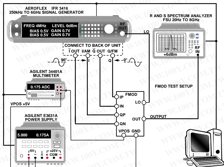
Figure 38. Characterization Bench Setup
