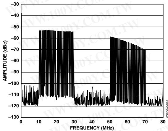
Figure 54. AD9861 Tx Path FFT of OFDM Signal in Figure 52, with 1x Interpolation
