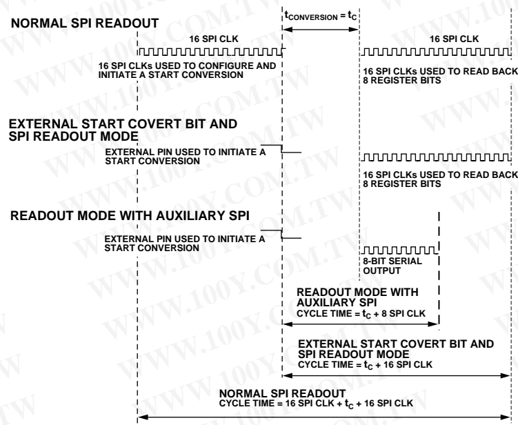
Figure 77. AuxADC Data Cycle Times for Various Readout Methods
