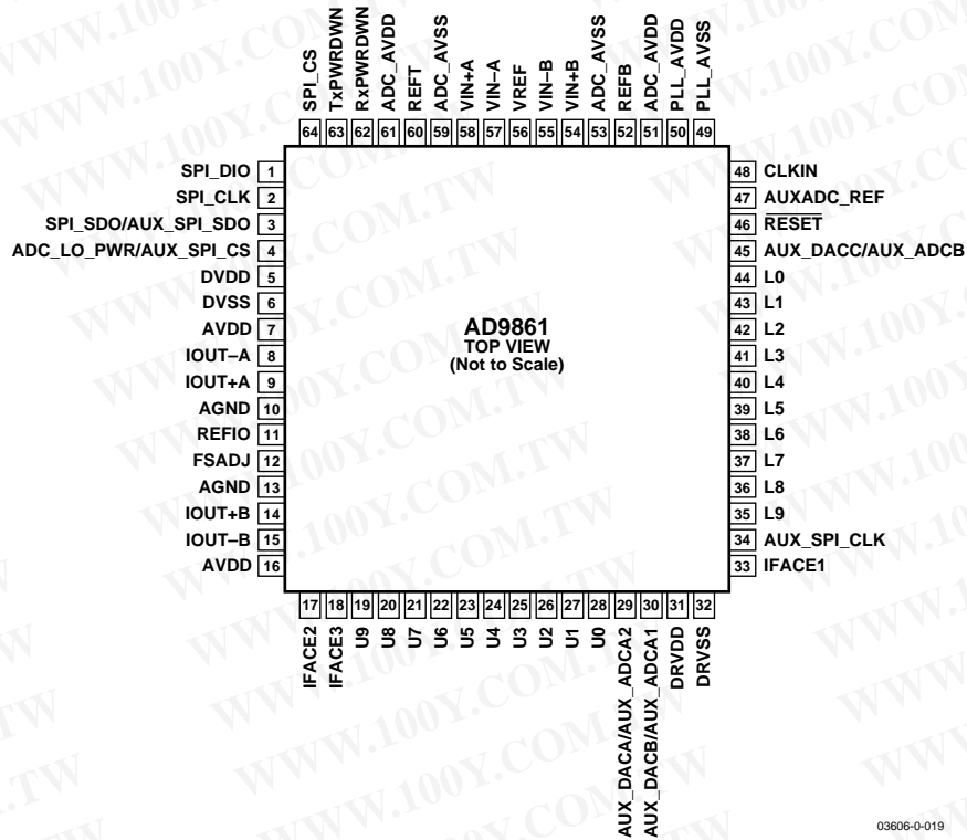
Figure 3. Pin Configuration
