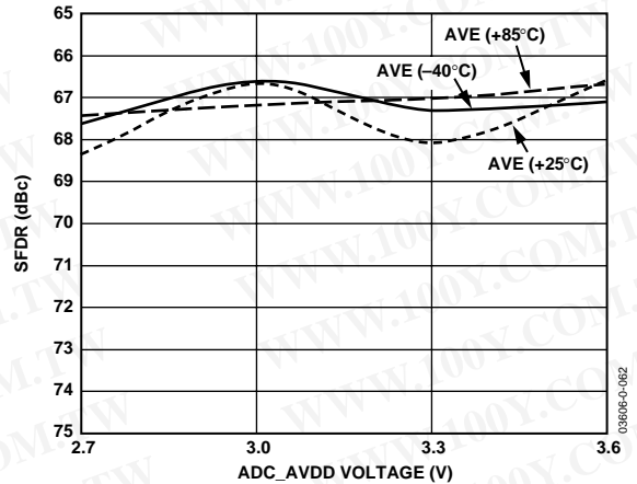
Figure 38. AD9861-80 Rx Path at 80 MSPS, 10 MHz Input Tone SFDR Performance vs. AVDD and Temperature
