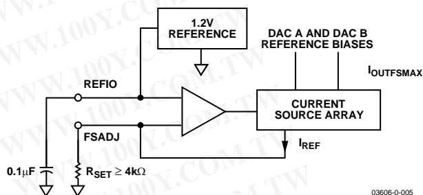
Figure 74. Reference Circuitry
