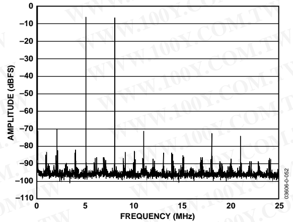
Figure 26. AD9861-80 Rx Path Dual-Tone FFT of Rx Channel A Path Digitizing 5 MHz and 8 MHz Tones
