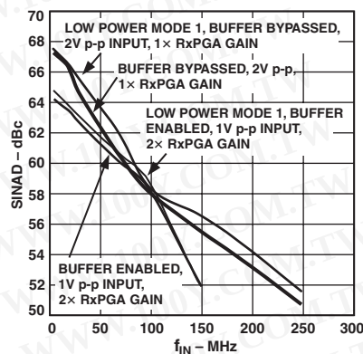
TPC 14. AD9862 Rx SINAD vs. f_{IN} at 32 MSPS
