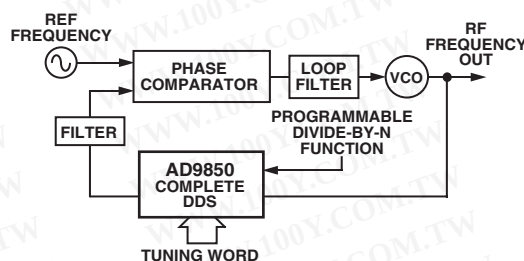
3c. Digitally-Programmable Divide-by-N Function in PLL
