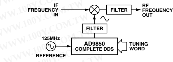
3a. Frequency/Phase-Agile Local Oscillator
