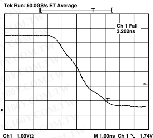
TPC 10. Comparator Output Fall Time (5 V Supply/15 pF Load)
