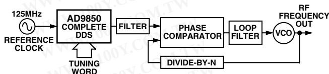
3b. Frequency/Phase–Agile Reference for PLL
