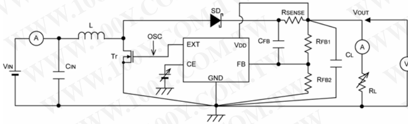
Circuit
