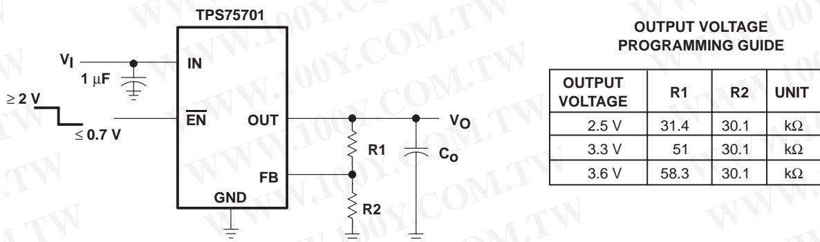
Figure 28. TPS75701 Adjustable LDO Regulator Programming
