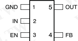
DBV Package (Top View) TPS72301
