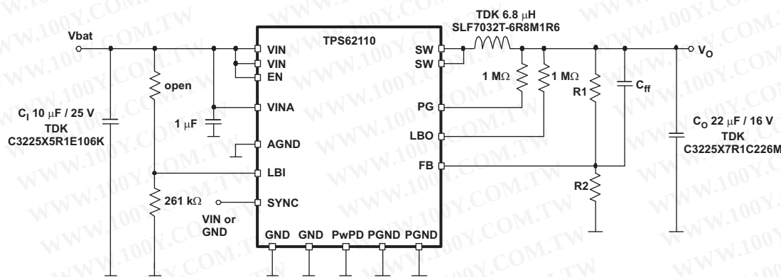
Figure 17. Test Setup
