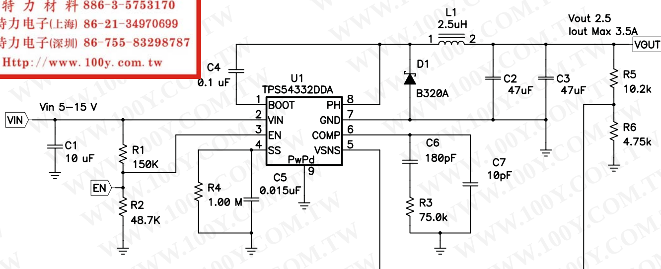
Figure 12. Typical Application Schematic
