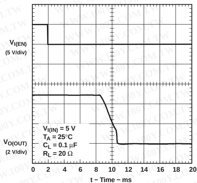
Figure 3. Turnoff Delay and Rise Time With 0.1-μF Load
