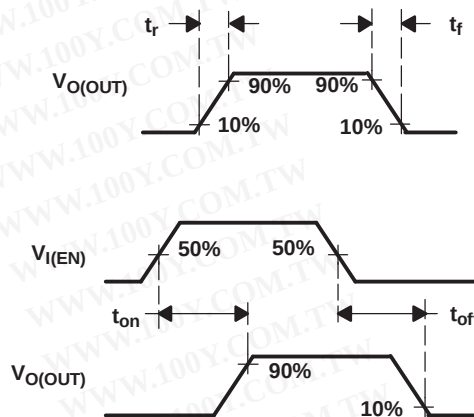
Figure 1. Test Circuit and Voltage Waveforms
