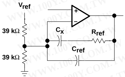
Test Circuit
