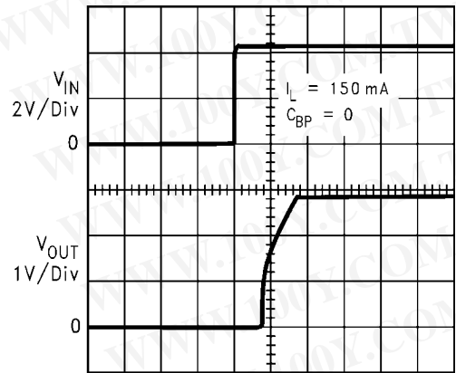
Startup Time ( V_{IN} = 4.2V )
