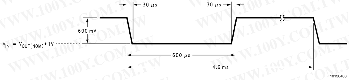
FIGURE 1. Line Transient Input Test Signal
