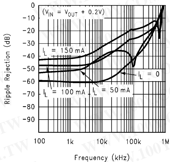
Ripple Rejection ( V_{IN} = V_{OUT} + 0.2V )
