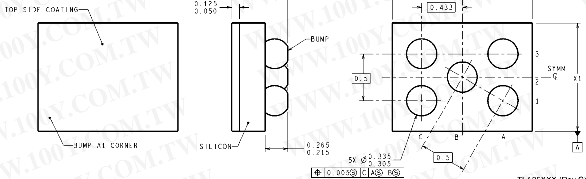
thin micro SMD, 5 Bump, Package (TLA05) NS Package Number TLA05AEA
