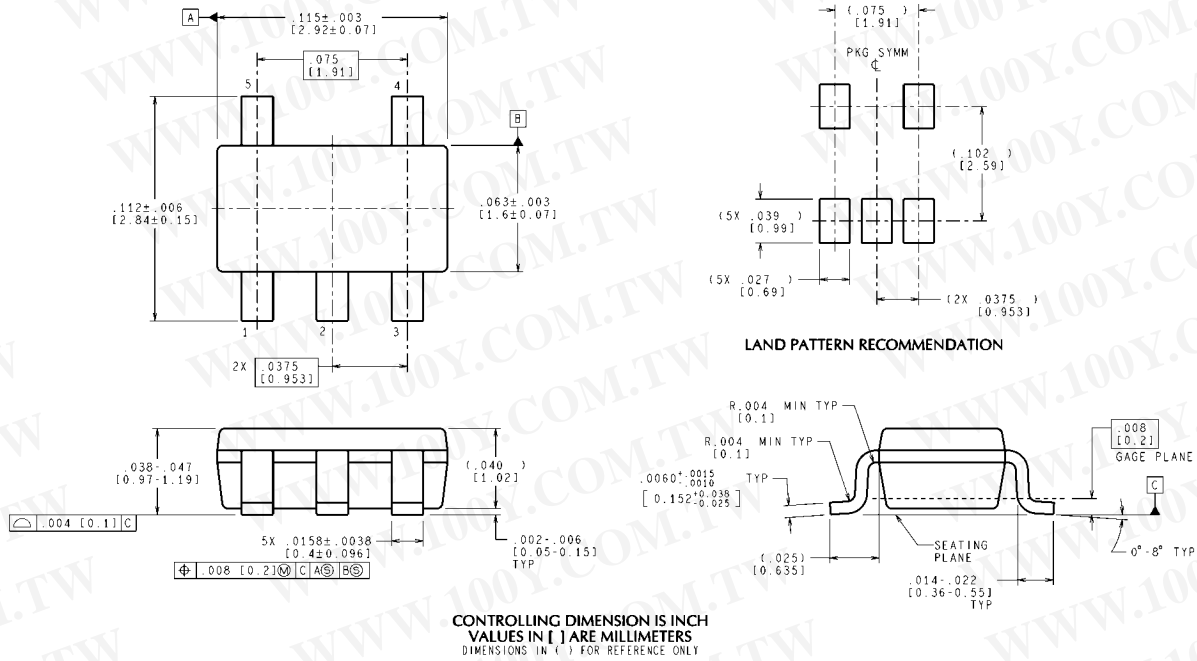
5-Lead Small Outline Package (MF) NS Package Number MF05A
