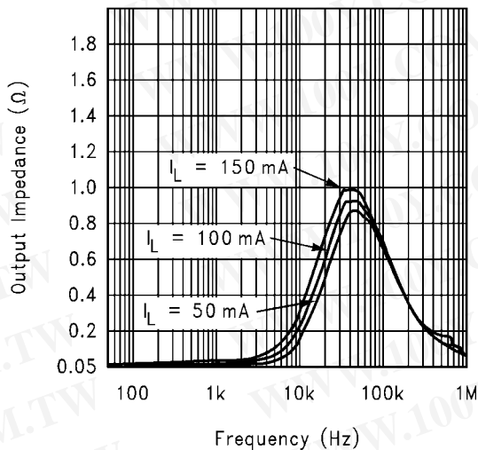
Output Impedance ( V_{IN} = 4.2V )
