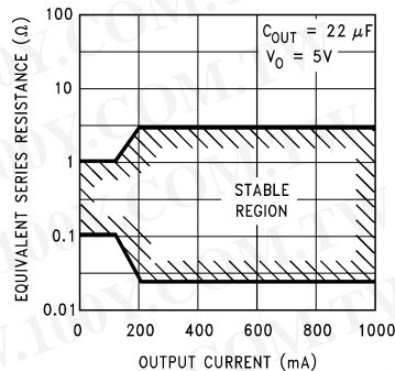
Figure 35. Output Capacitor ESR Limits
