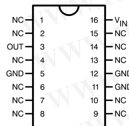
Figure 4. 16-Lead CLGA (NAC) Top View See Package Number NAC0016A
