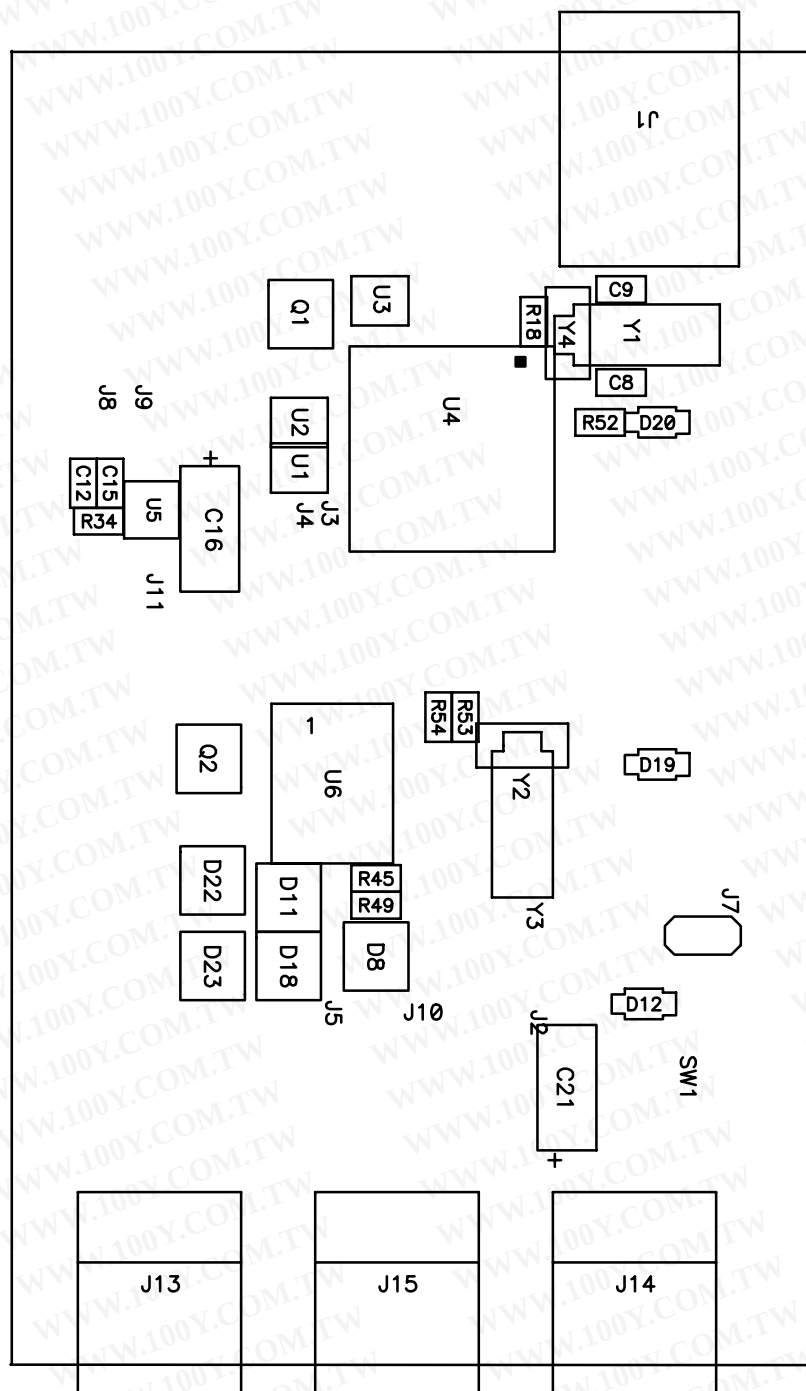
Figure 3-5. Component Placement 1
