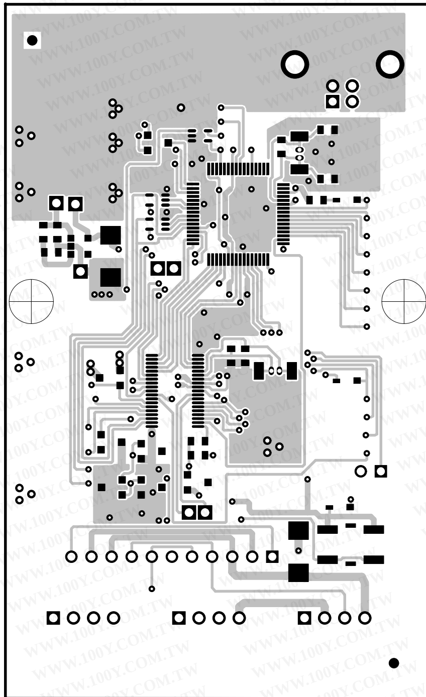
Figure 3–1. Board Layer 1
