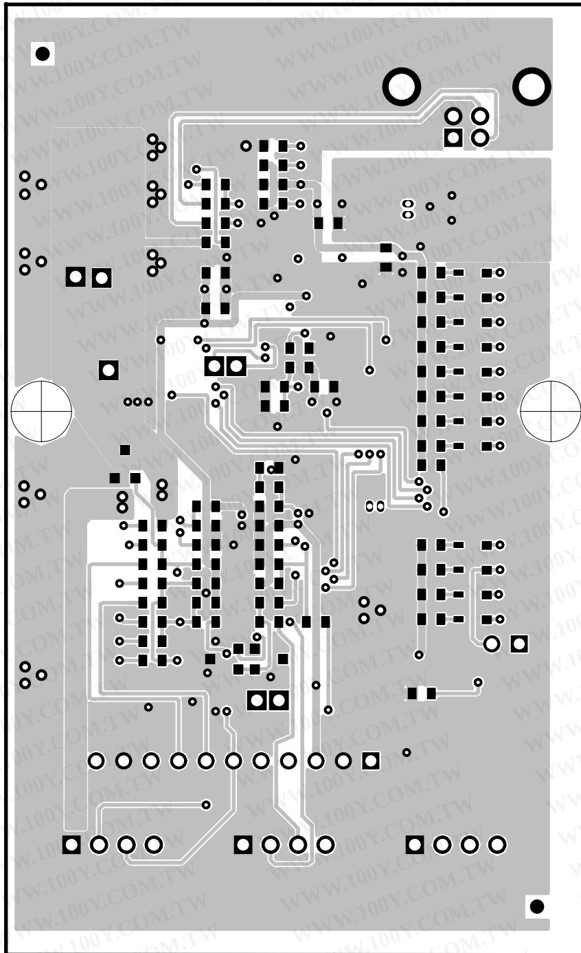
Figure 3-4. Board Layer 2
