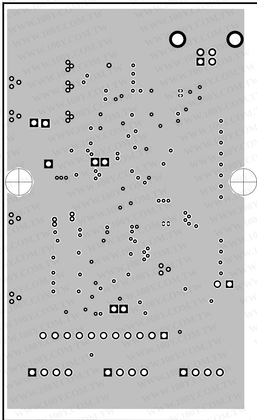
Figure 3-7. Internal Board Layer 1
