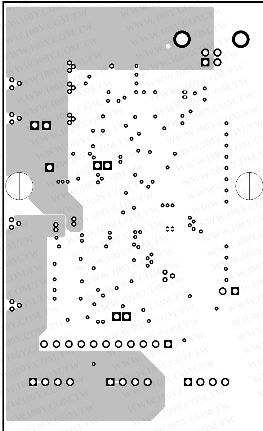
Figure 3-8. Internal Board Layer 2
