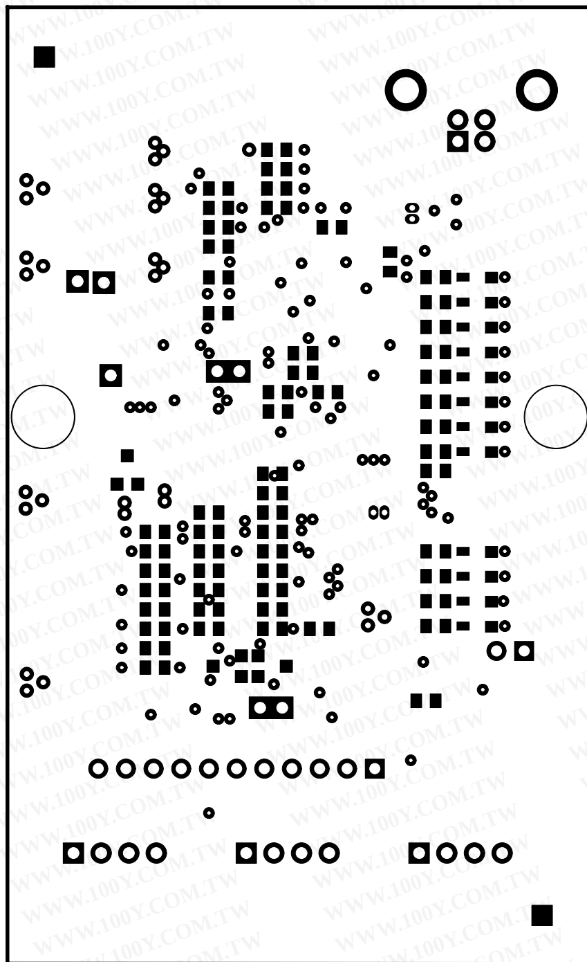
Figure 3-3. Solder Mask 2
