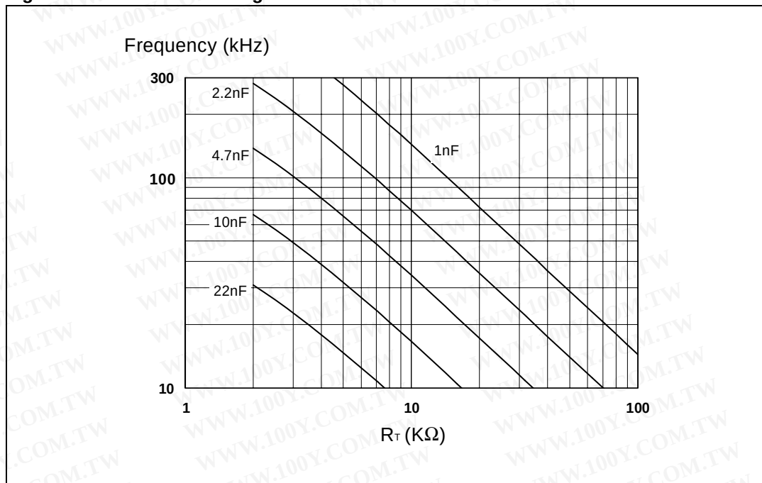
Figure 16. Oscillator Settings
