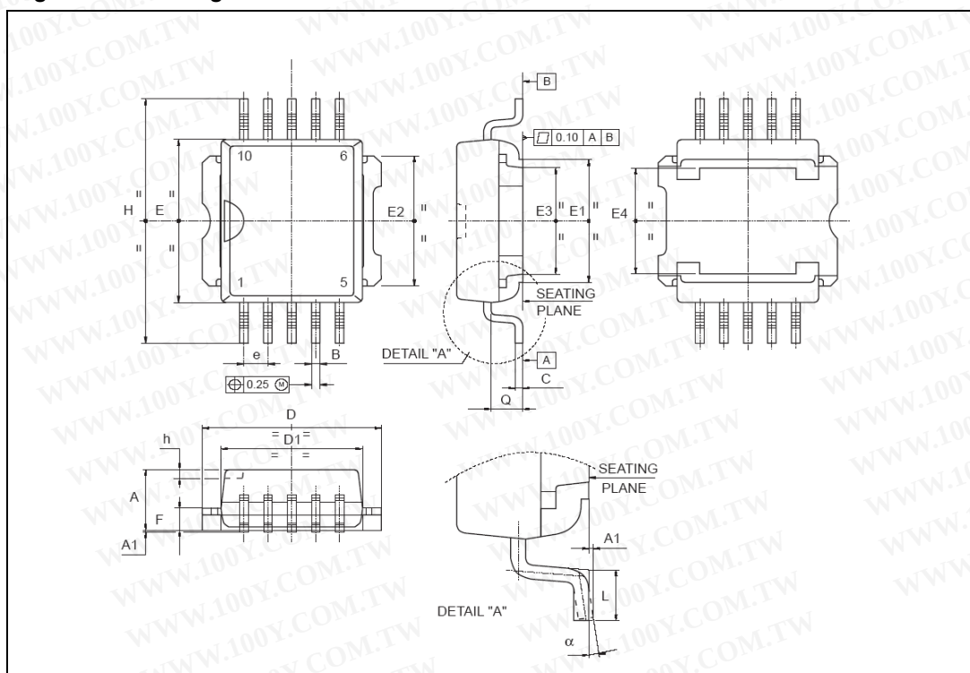
Figure 20. Package Dimensions
