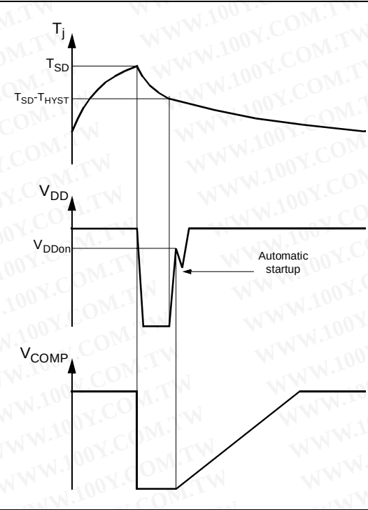
Figure 11. Thermal Shutdown
