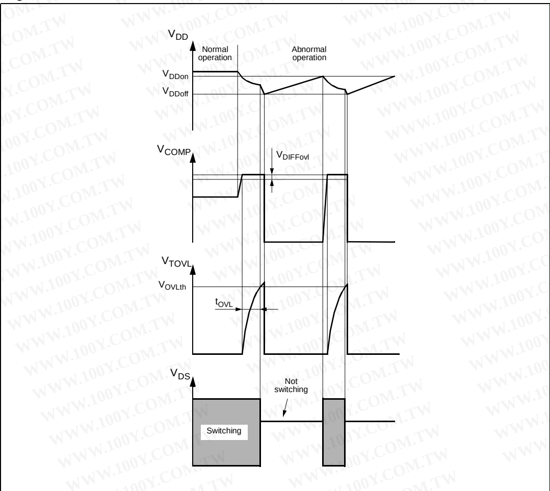
Figure 7. Overloaded Event
