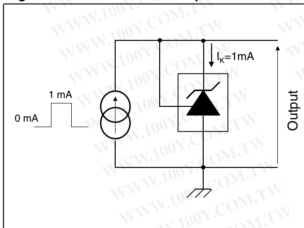
Figure 10. Test circuit for response time
