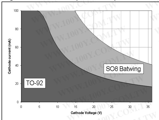
Figure 21. Maximum power dissipation
