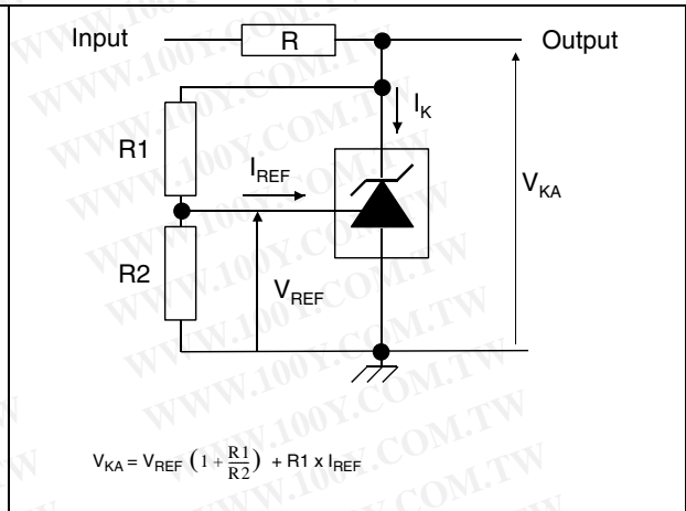
Figure 7. Test circuit for programming mode
