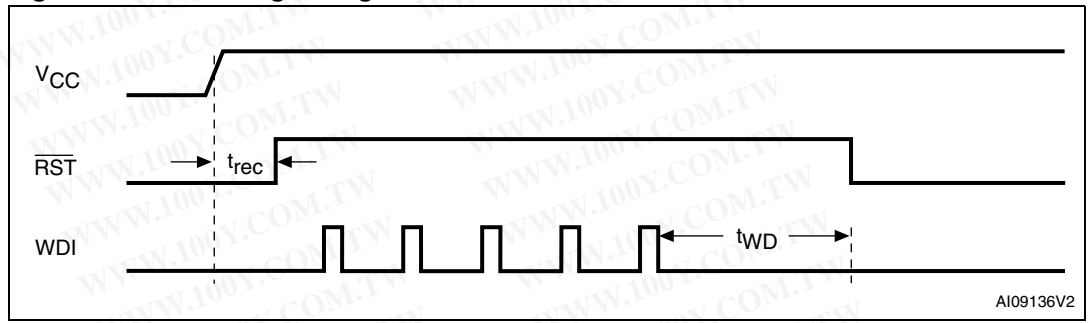
Figure 26. Watchdog timing
