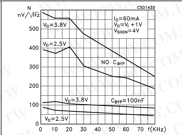
Figure 22. Spectrum noise
