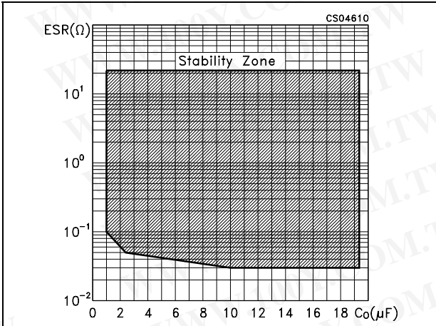
Figure 21. Stability
