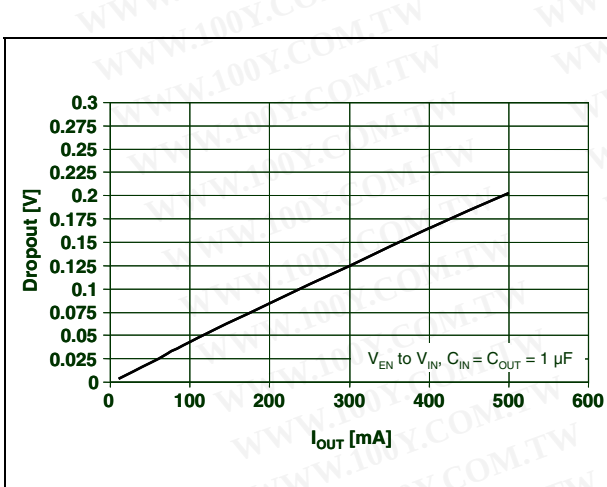
Figure 8. Dropout voltage vs. output current
