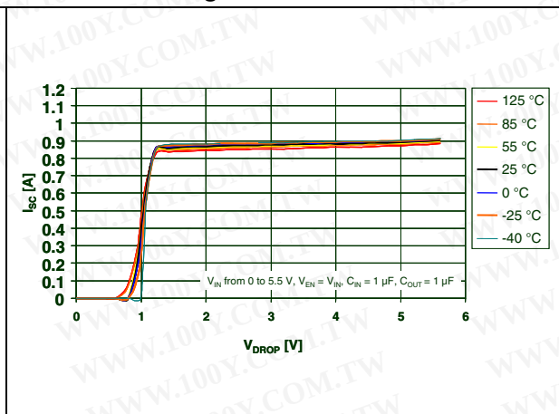
Figure 9. Short-circuit current vs. dropout voltage
