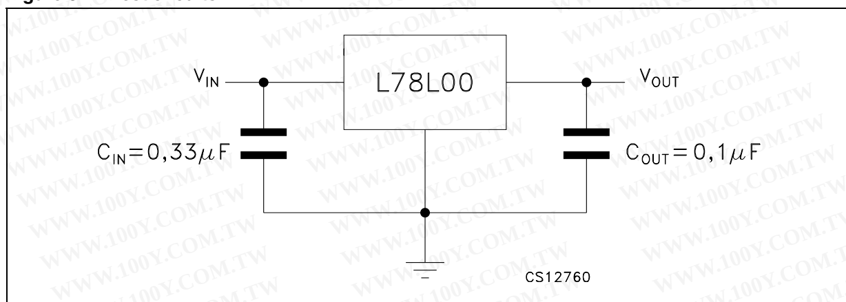
Figure 3. Test circuits
