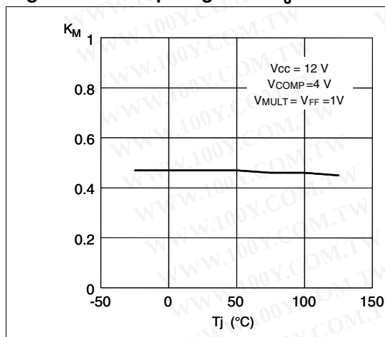
Figure 20. Multiplier gain vs T_J
