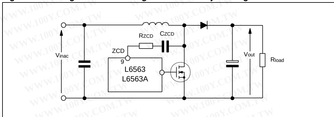
Figure 54. Demagnetization sensing without auxiliary winding
