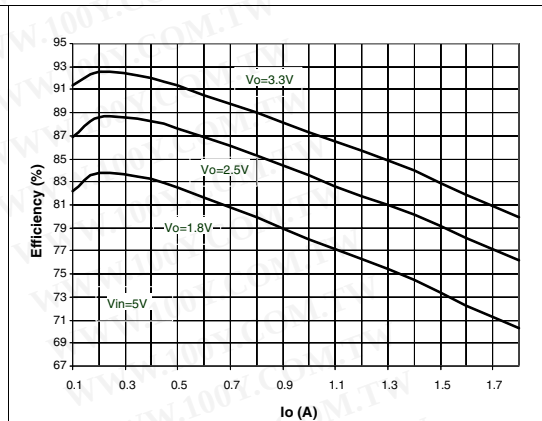
Figure 16. Efficiency vs output current
