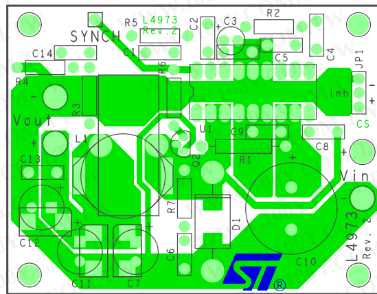
Figure 5. Evaluation board (components side)
