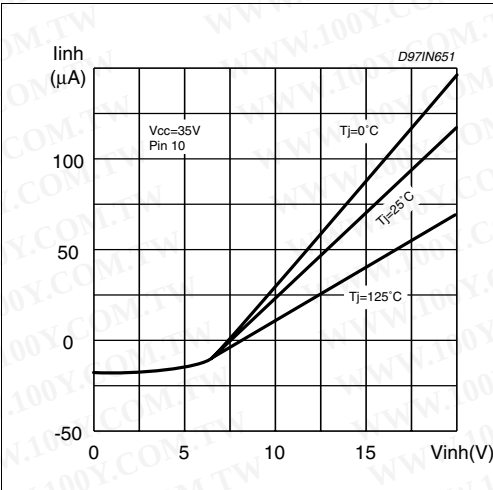
Figure 15. Inhibit current vs. inhibit voltage (pin 10)
