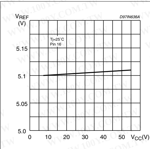
Figure 13. Reference voltage vs. input voltage (pin 16)
