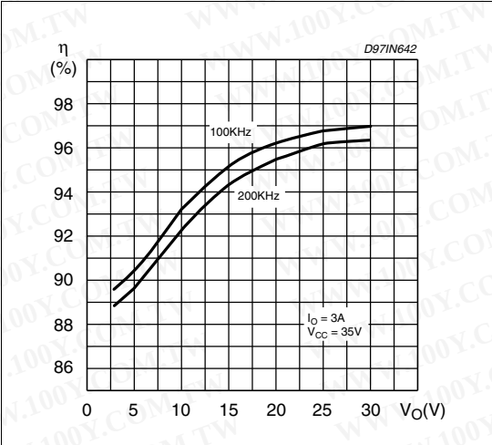
Figure 27. Efficiency vs. output voltage (Diode STPS745D)
