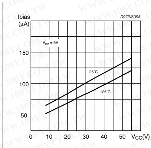
Figure 11. Stand by drain current vs. input voltage
