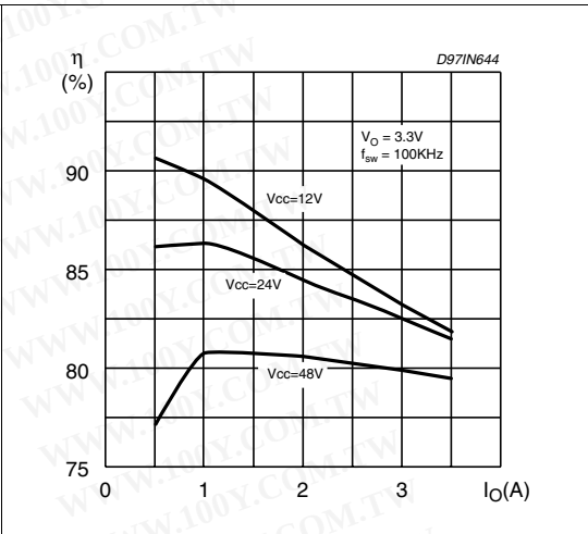
Figure 30. Efficiency vs. output current (see Figure 8)
