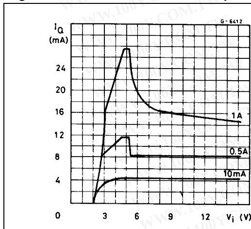
Figure 10. Quiescent current vs input voltage
