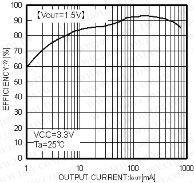
Fig.74 Efficiency
