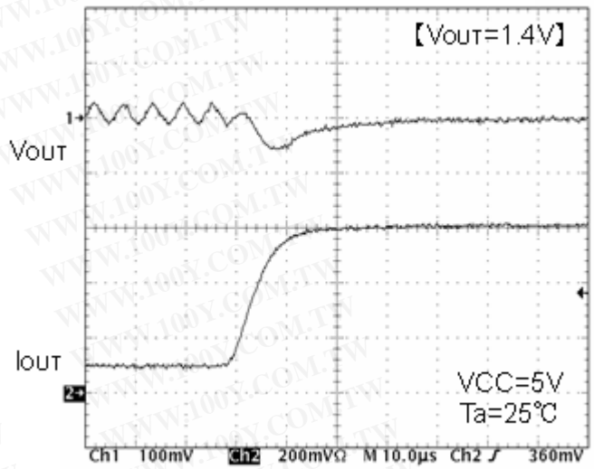
Fig. 68 Transient response Io=100→600mA(10μs)
