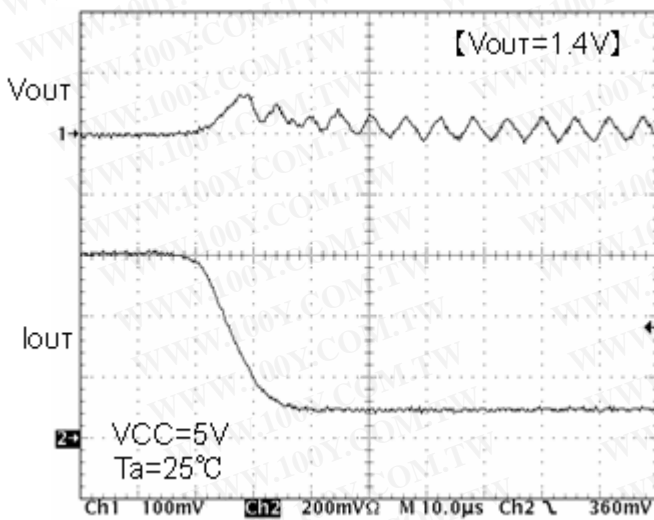
Fig.69 Transient response Io=600→100mA(10μs)
