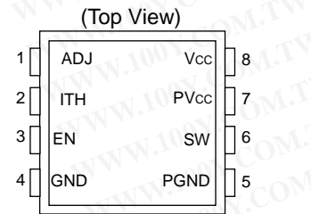
Fig.5 BD9120HFN
