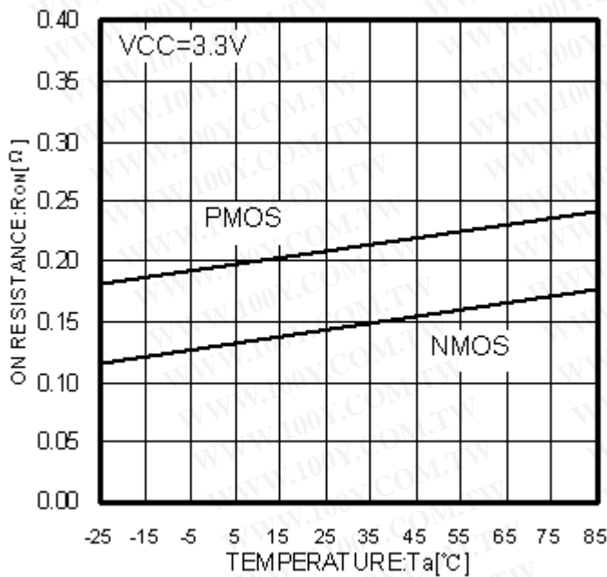
Fig.76 Ta-Ronn, Ronp
