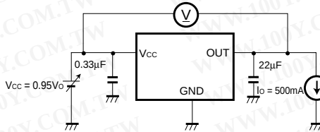
Fig. 3 Measurement circuit for minimum I/O voltage differential
