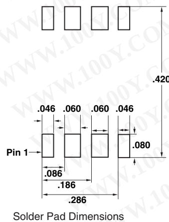
Solder Pad Dimensions
