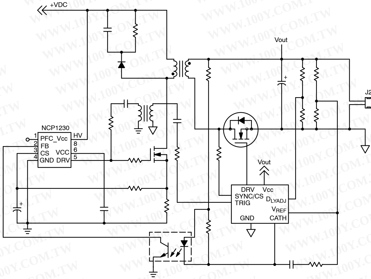
Figure 2. Typical Application
