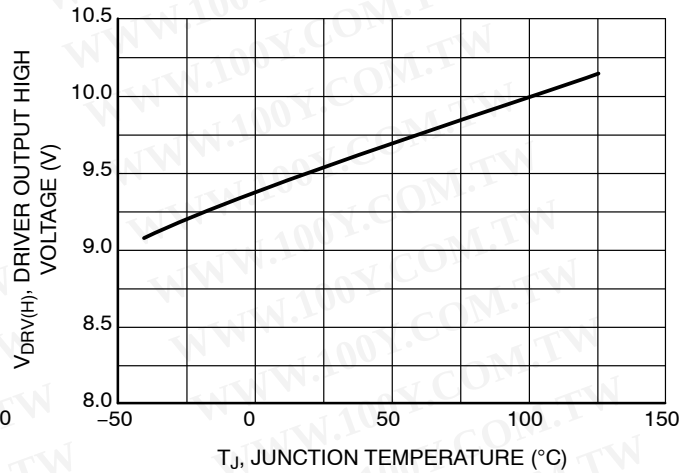
Figure 8. Driver V out High vs. Junction Temperature
