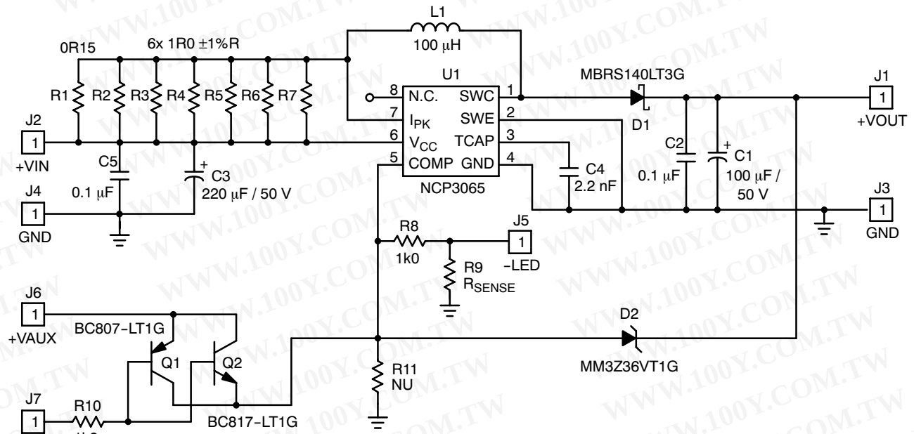
Figure 22. Boost Demo Board Application Schematic
