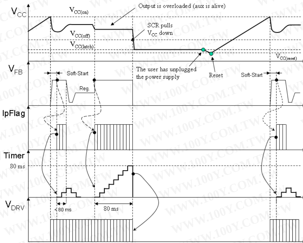
Figure 39. Latched Short-Circuit Protection on A and C Versions
