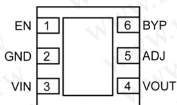
MIC5319BML/YML (Adjustable) 6-Pin 2mm × 2mm MLF ® (ML) Top View
