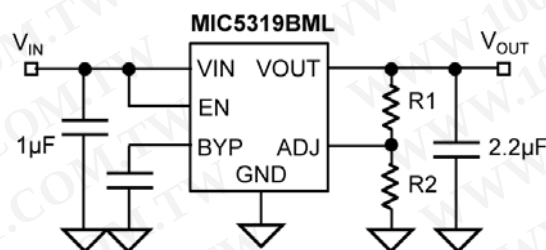
Figure 1. Adjustable Voltage Application
