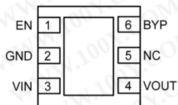
MIC5319-x.xBML/YML 6-Pin 2mm × 2mm MLF ® (ML) Top View
