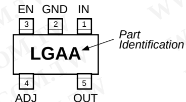
MIC5219BM5 SOT-23-5 Adjustable Voltage
