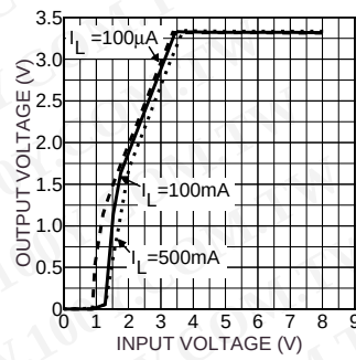
Dropout Characteristics
