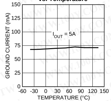
MIC2950x Ground Current vs. Temperature
