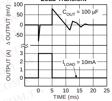
MIC2930x Load Transient
