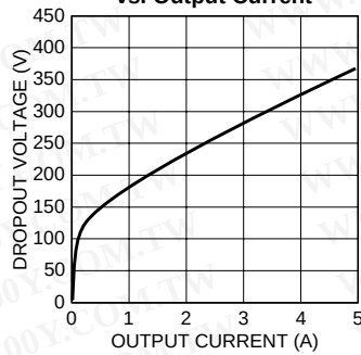
MIC2950x Dropout Voltage vs. Output Current
