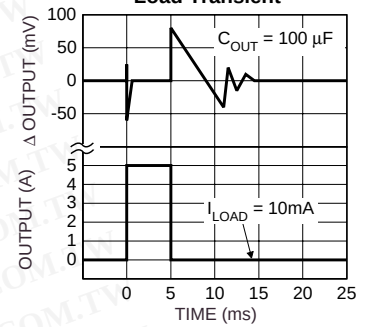
MIC2950x Load Transient
