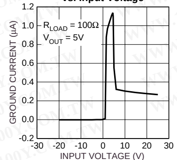
MIC2915x Ground Current vs. Input Voltage
