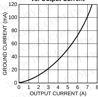
MIC2975x Ground Current vs. Output Current
