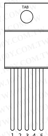
MIC29201/29202BT (TO-220-5)
