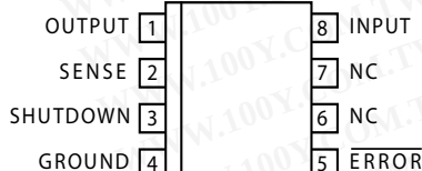
MIC29201-3.3BM (SOIC-8)
