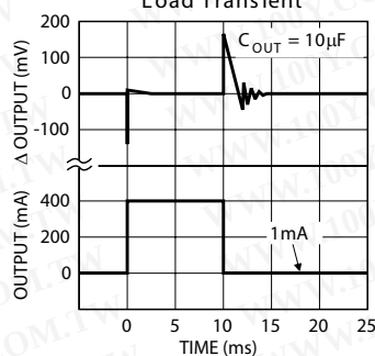
Load Transient
