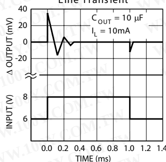
Line Transient
