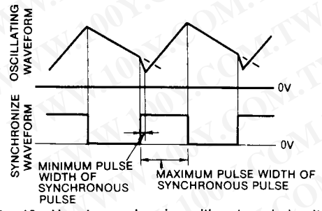
Fig. 46 How to synchronize with external circuit
