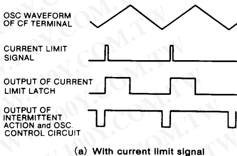
(a) With current limit signal
