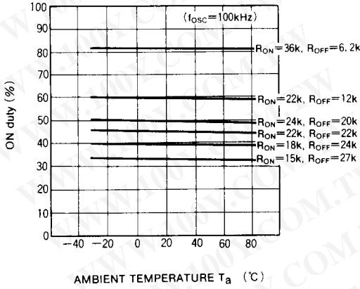
ON duty VS. AMBIENT TEMPERATURE
