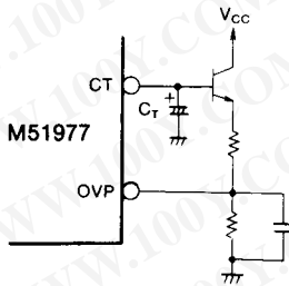
Fig. 39 Application circuit diagram to keep the non-operating condition when over load current condition will continue for specified duration
