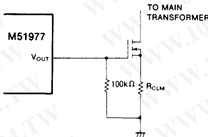
Fig. 40 Circuit diagram to prevent the MOS-FET gate potential rising
