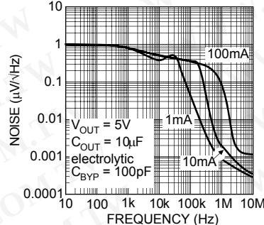
Noise Performance
