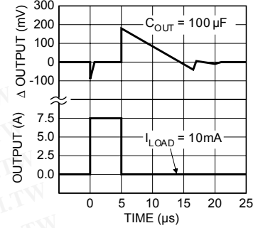
MIC2975x Load Transient
