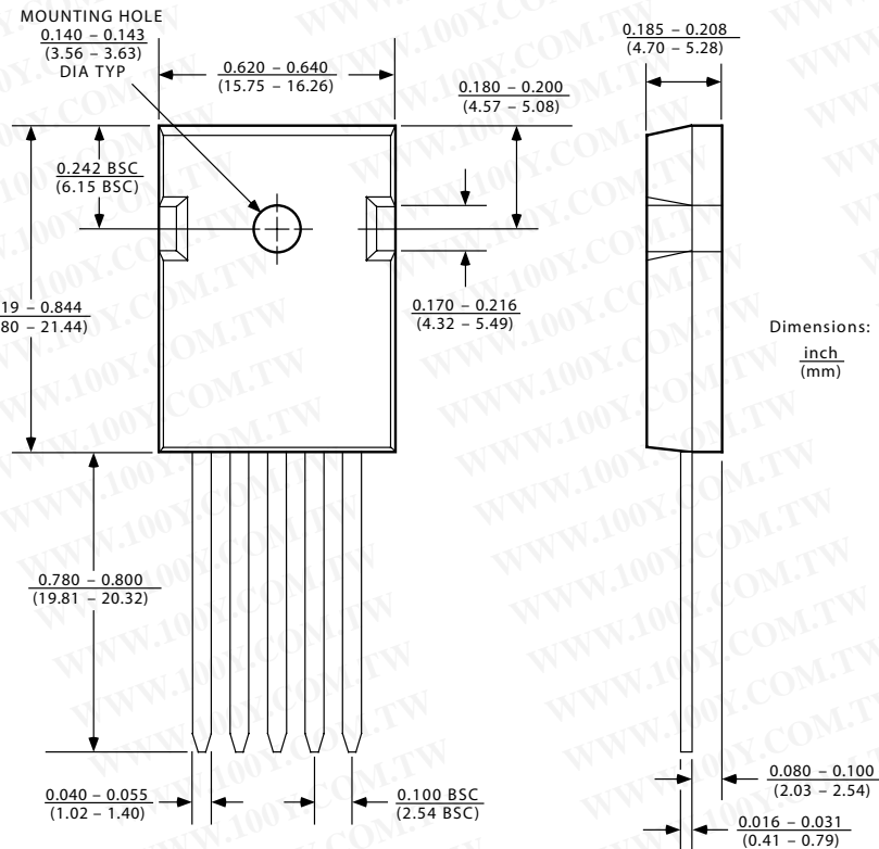
5-Lead TO-247 (W)
