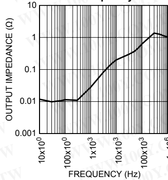
MIC2915x Output Impedance vs. Frequency
