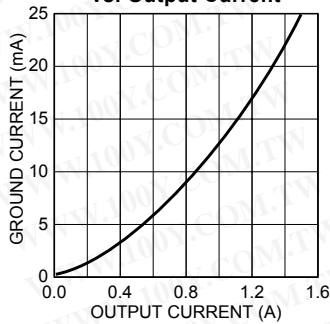
MIC2915x Ground Current vs. Output Current
