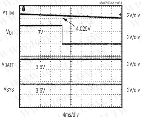
THM NORMAL TO THM HOT THRESHOLD DISCHARGE T_{OT} MAX8934A t0c34
