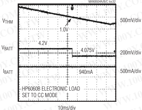
THM NORMAL TO THM HOT (> T3) TRANSITION MAX8934A/B/C t0c32
