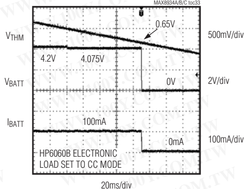
THM NORMAL TO THM HOT NO CHARGE (> T4) TRANSITION MAX8934A/B/C t0c33
