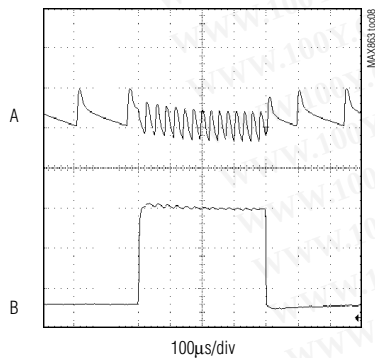
LOAD-TRANSIENT RESPONSE
