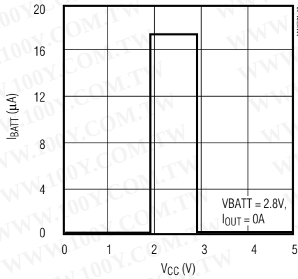
BATTERY CURRENT vs. INPUT SUPPLY VOLTAGE
