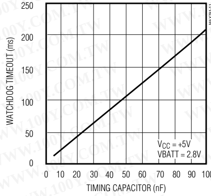
WATCHDOG TIMEOUT vs. TIMING CAPACITOR
