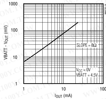
V_{BATT} to V_{OUT} vs. OUTPUT CURRENT
