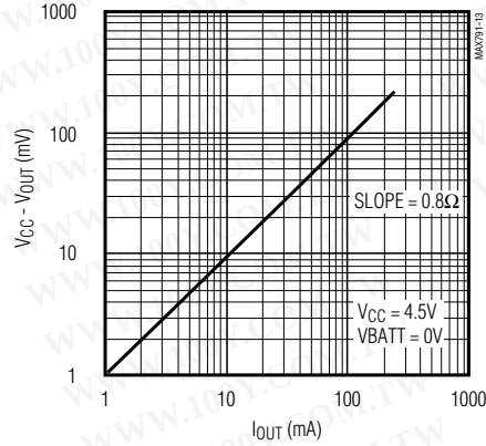
V_{CC} to V_{OUT} vs. OUTPUT CURRENT
