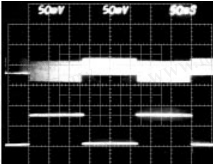
MAX730A LOAD-TRANSIENT RESPONSE
