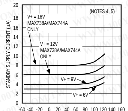
STANDBY SUPPLY CURRENT vs. TEMPERATURE
