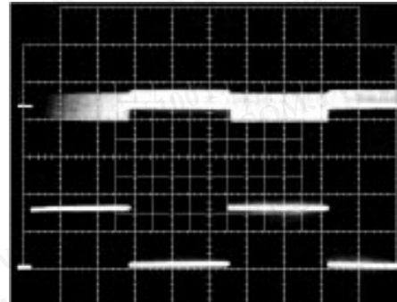
MAX738A/MAX744A LOAD-TRANSIENT RESPONSE
