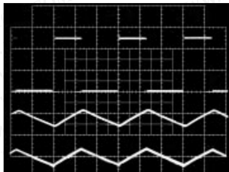
MAX738A/MAX744A SWITCHING WAVEFORMS, CONTINUOUS CONDITION
